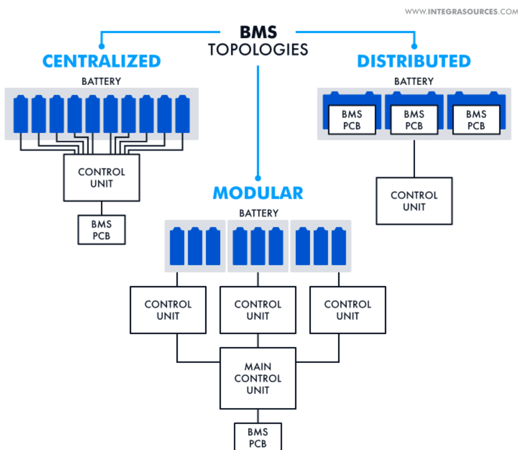
Figure 2.1 Different BMS architectures.
